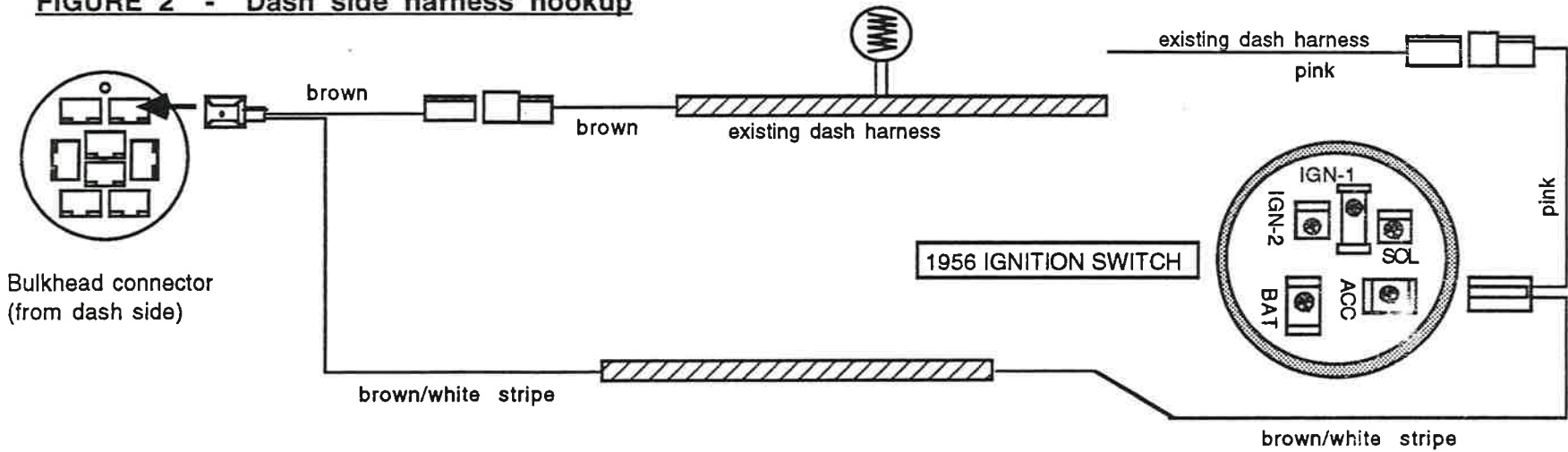
FIGURE 2 - Dash side harness hookup
